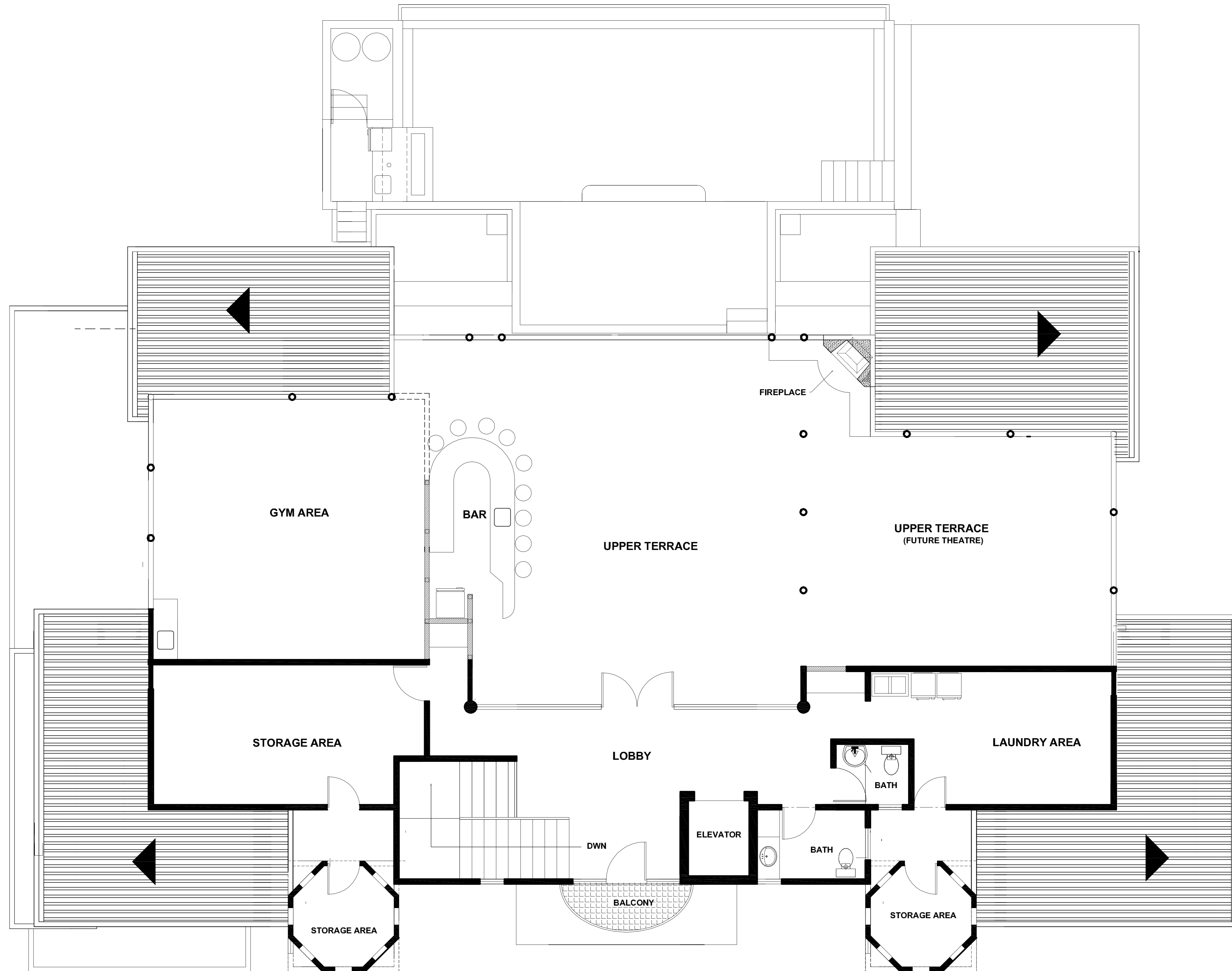
THIRD LEVEL PLAN
